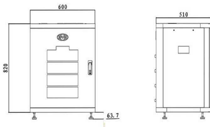
Structure dimension drawing
