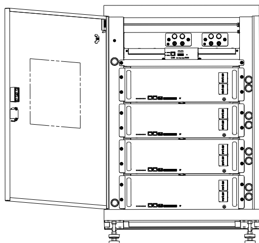
Internal drawing
